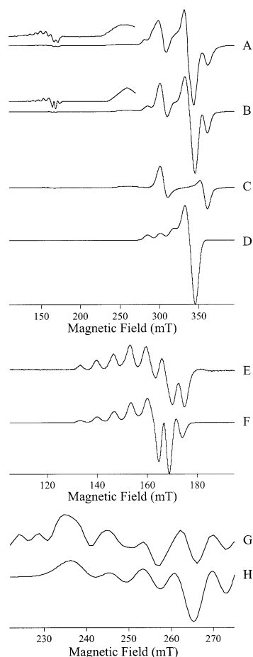
Figure 5. EPR simulations of the signals from [CuCu(AAP)]. Trace A shows the B_1 \perp B_0 EPR signal from [CuCu(AAP)] at pH 9.65 recorded at 45 K, 2 mW microwave power, and 1.0 mT magnetic field modulation amplitude. The low-field region of the spectrum is shown multiplied by a factor of 9 above the main trace. Trace B shows a simulation obtained by addition of traces C and D. The low-field region of the simulation is shown multiplied by a factor of 9 above the main trace. Trace C is an Xsophe simulation assuming a dinuclear copper system, using the spin Hamiltonian and associated parameters \mathcal{H} = \beta\mathbf{B} \cdot \mathbf{g}_{\text{CuA}} \cdot \mathbf{S}_{\text{CuA}} + \beta\mathbf{B} \cdot \mathbf{g}_{\text{CuB}} \cdot \mathbf{S}_{\text{CuB}} + [\mathbf{S}_{\text{CuA}} \cdot \mathbf{A} \cdot \mathbf{I}]_{\text{CuA}} + [\mathbf{S}_{\text{CuB}} \cdot \mathbf{A} \cdot \mathbf{I}]_{\text{CuB}} + [\mathbf{S}_{\text{CuA}} \cdot \mathbf{J} \cdot \mathbf{S}_{\text{CuB}}] ; g_{\parallel(\text{CuA,CuB})} = 2.218 and g_{\perp(\text{CuA,CuB})} = 2.060 ; A_{\parallel(\text{CuA,CuB})(^{63/65}\text{Cu})} = 1.59 \times 10^{-2} \text{ cm}^{-1} and A_{\perp(\text{CuA,CuB})(^{63/65}\text{Cu})} = 2.0 \times 10^{-3} \text{ cm}^{-1} ; J_{\text{isotropic}} = 50 \text{ cm}^{-1} ; r_{\text{CuA-CuB}} = 4.93 \text{ \AA} and \chi = 17^\circ . Trace D is a simulation assuming an isolated Cu(II) ion with g_{\parallel} = 2.218 , g_{\perp} = 2.023 , and A_{\parallel(^{63/65}\text{Cu})} = 1.55 \times 10^{-2} \text{ cm}^{-1} . Trace E is a higher resolution spectrum of [CuCu(AAP)] at pH 9.65, recorded at 45 K, 2 mW microwave power, and 0.25 mT magnetic field modulation amplitude. Trace F is an expanded version of trace B over the magnetic field range corresponding to trace E. Trace G is the third derivative ( \partial^3\chi''/\partial H^3 ) spectrum of [CuCu(AAP)] over a narrow field range. Trace H is the corresponding simulation of G using the parameters for trace C.
