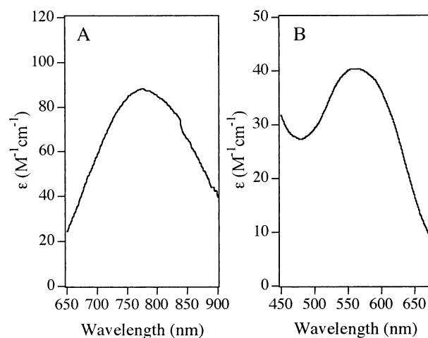
Figure 1. Electronic absorption spectra of (A) [CuCu(AAP)] and (B) [Cu 1 EcMetAP ] at pH 7.5.
