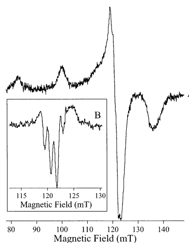
Figure 8. S-Band EPR of [Cu_(MAP)]. (A) EPR spectrum of [Cu_(MAP)] at pH 6.8 recorded at 90 K, 3.43 GHz and 0.4 mT magnetic field modulation amplitude and with 15 dB microwave power attenuation. (B) Second derivative spectrum ( \partial^2\chi''/\partial H^2 ) of the g_{\perp} region.
