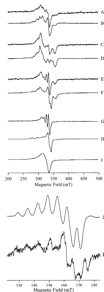
Figure 7. EPR spectra of Cu(II) added to apo-AAP. The traces A–H show spectra from solutions of 50 mM Tris-HCl buffer, pH 7.0, containing AAP and Cu(II) at the following concentrations: (A and B) 2.7 mM AAP, 2.7 mM Cu(II); (C and D) 2.0 mM AAP, 4.0 mM Cu(II); (E and F) 1.6 mM AAP, 4.8 mM Cu(II); and (G and H) 1.3 mM AAP, 5.2 mM Cu(II). Trace I corresponds to 5 mM Cu(II) in the absence of AAP. Trace J corresponds to trace E of Figure 5 and is shown for comparison. Spectrum K is from the same sample as for spectra C and D shown here. Spectra A, C, E, and G were recorded at 295 \pm 3 \text{ K} and 10 mW microwave power. Spectra B, D, F, H, I, and K were recorded at 12 K and 1.0 mW microwave power. All spectra were recorded using a Bruker ER 4116 DM cavity containing a quartz dewar insert and with the sample capillary mounted inside a 3 mm diameter EPR tube containing 100 \mu\text{L} of ethanol to facilitate thermal contact at low temperature. Spectra were recorded with 0.5 mT field modulation amplitude.
