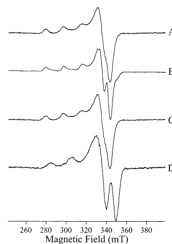
Figure 2. EPR signals from [Cu 1 (AAP)] and [Cu 1 ( EcMetAP )]. (A) [Cu 1 (AAP)] at pH 6.0, (B) [Cu 1 (AAP)] at pH 9.65, (C) [Cu 1 ( EcMetAP )] at pH 6.8, and (D) [Cu 1 ( EcMetAP )] at pH 10.1. Spectra were recorded at 45 K, 2 mW microwave power, and 0.25 mT magnetic field modulation amplitude.
