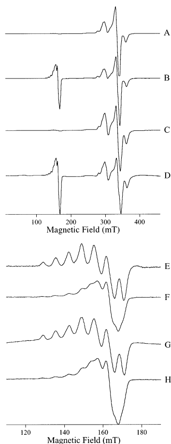
Figure 3. EPR signals from [CuCu(AAP)]. The top two traces show the EPR spectra from [CuCu(AAP)] at pH 6.0, recorded with (A) B_1 \perp B_0 and (B) B_1 \parallel B_0 . The bottom two traces show the EPR spectra from [CuCu(AAP)] at pH 9.65 recorded with (C) B_1 \perp B_0 and (D) B_1 \parallel B_0 . Traces E–H show high-resolution spectra of A–D, respectively, recorded over the field range indicated by the scales. Spectra A, B, E, and F were recorded at 45 K and 2 mW microwave power, and spectra C, D, G, and H were recorded at 4 K and 0.5 mW microwave power. Spectra A–D were recorded with 1.0 mT magnetic field modulation amplitude and spectra E–H with 0.25 mT magnetic field modulation amplitude. Spectra are shown with normalized intensities.
