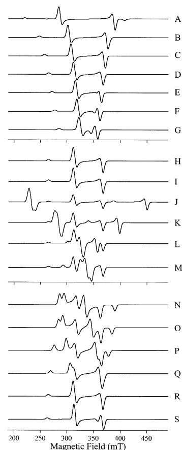
Figure 6. Calculated spectra assuming two spin-coupled S = 1/2 axial species. The individual species were calculated assuming identical g values for the individual species, g_{\parallel} = 2.2 and g_{\perp} = 2.0 , with line widths of 3.0 mT. For simplicity, no hyperfine interaction was considered. Spectra A–G illustrate the effect of varying the dipolar coupling as a function of the intercenter distance, r . Spectra were calculated for (A) r = 4.25 \text{ \AA} , (B) 4.50 Å, (C) 4.75 Å, (D) 5.00 Å, (E) 5.25 Å, (F) 5.50 Å, and (G) 6.00 Å. For spectra A–G, J_{\text{isotropic}} = 5 \text{ cm}^{-1} and \chi = 17^\circ . Spectra H–M illustrate the effect of J_{\text{isotropic}} assuming a fixed dipolar coupling. The values of J_{\text{isotropic}} used were (H) 5 \text{cm}^{-1} , (I) 0.5 \text{cm}^{-1} , (J) 0.1 \text{cm}^{-1} , (K) 5 \times 10^{-2} \text{ cm}^{-1} , (L) 1 \times 10^{-2} \text{ cm}^{-1} , and (M) 0. For all spectra H–M, r = 5.00 \text{ \AA} and \chi = 17^\circ . Spectra N–S illustrate the effect of varying the angle, \chi , between the dipolar coupling vector and g_z . Spectra were calculated for \chi = 90^\circ (N), 60^\circ (O), 45^\circ (P), 30^\circ (Q), 17^\circ (R), and 0^\circ (S). For spectra N–S, r = 5.00 \text{ \AA} and J_{\text{isotropic}} = 5 \text{ cm}^{-1} .
