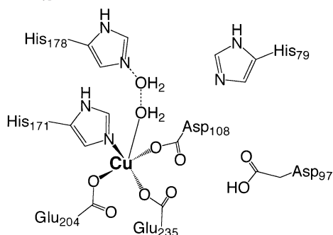
Chart 2. Proposed Structure of the Metal Binding Site in [Cu 1 ( EcMetAP )]
